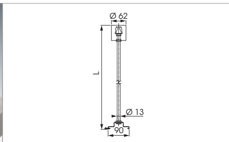
Pendant tubing. 2 units for single-length luminaires, minimum of 2 units for double-length luminaires, minimum of 3 units for triple-length luminaires.
