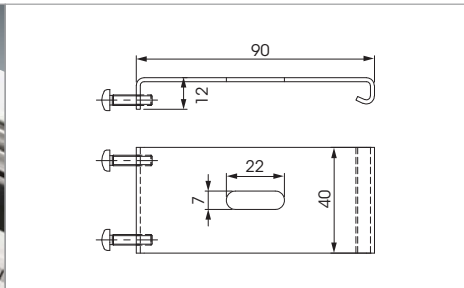
Ceiling mounting bracket. 2 units for single-length luminaires, minimum of 2 units for double-length luminaires, minimum of 3 units for triple-length luminaires.
