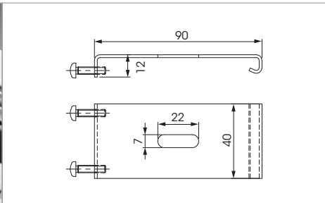
Ceiling mounting bracket. 2 units for single-length luminaires, minimum of 2 units for double-length luminaires, minimum of 3 units for triple-length luminaires.
