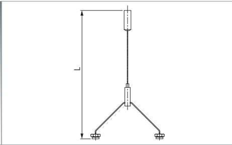
Three-point cable suspension. 2 units for single-length luminaires, minimum of 2 units for double-length luminaires, minimum of 3 units for triple-length luminaires.
