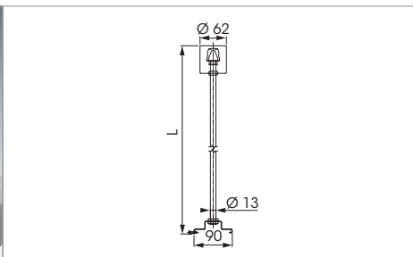
Pendant tubing. 2 units for single-length luminaires, minimum of 2 units for double-length luminaires, minimum of 3 units for triple-length luminaires.
