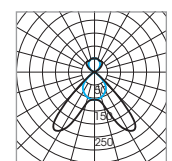
1 x T5 η=50%
