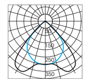
1 x T5 η=62%
