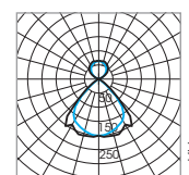
2 x T5 η=55%
